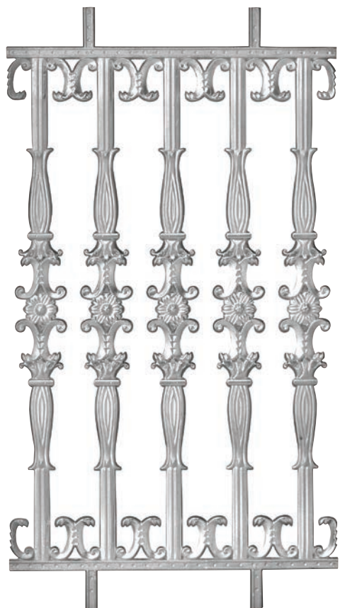
BALAÚSTRE | REF. ML 782 MED. 925(805)x510
