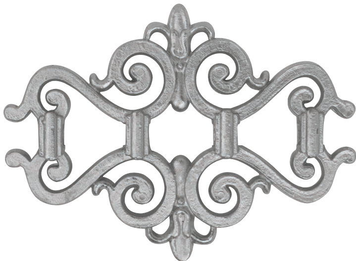
FLOR | REF. ML 283 MED. 280x208 F. \square 16
