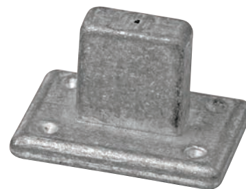
SAPATA | REF. ML 855 MED. 45x70x50 P/Tubo 40x20 MED. 45x60x40 P/Tubo 30x20 MED. 45x60x40 P/Tubo 30x15 MED. 45x60x40 P/Tubo 30x25
